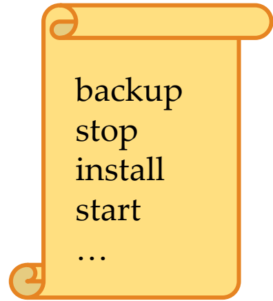
Deployment Script
